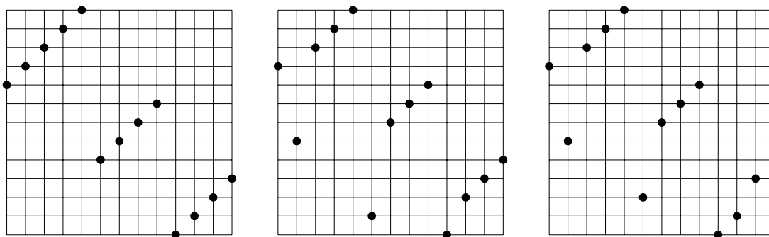
FIGURE 1. Permutations \tau_{3,13} , \sigma_3^1 , and \sigma_3^2 .
