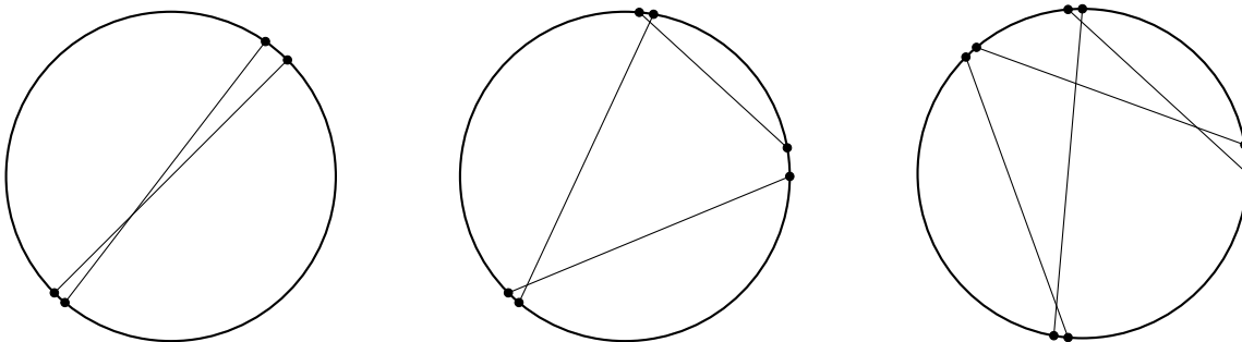
Figure 4.1: 2, 3 and 4-crossings.
