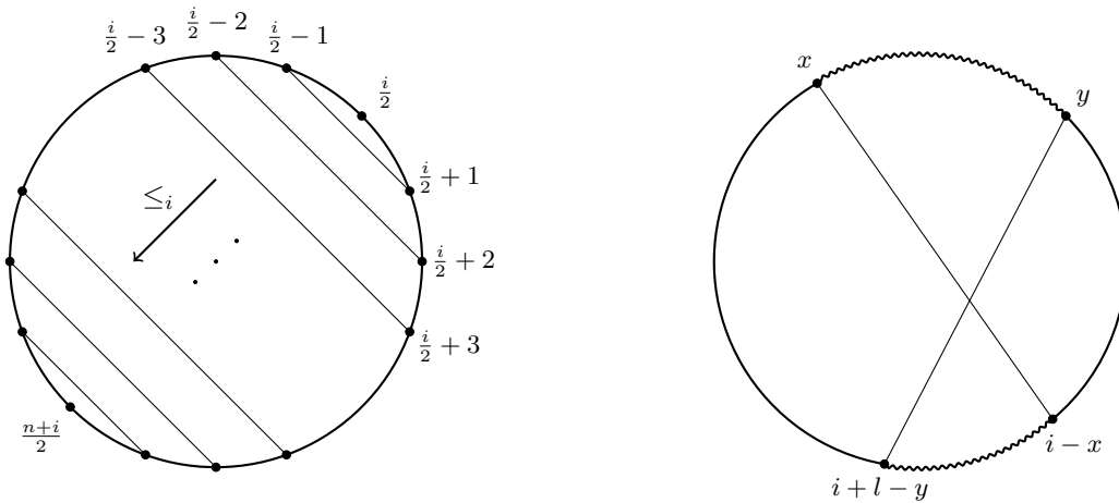
Figure 3.2: The set E_i in the case when both i and n are even, the arrow points from \leq_i -smaller to \leq_i -larger elements; a crossing between an edge \{x, i - x\} \in E_i and an edge \{y, i + l - y\} \in E_{i+l} , marked is the cycle of length l + 2 .
