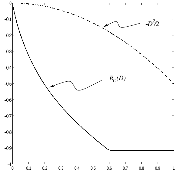
Fig. 1. Graph of the function R_C(D) = R(D; P, P) for 0 \leq D \leq 1 , in the case of the binary cube A^n = \{0, 1\}^n , with P(1) = 0.4 .
