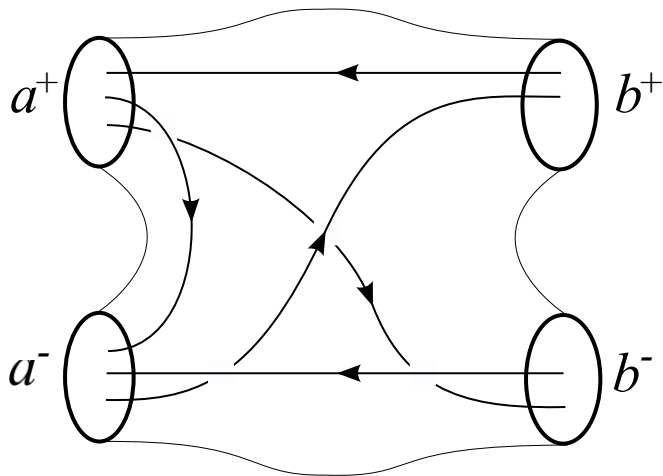
Figure: The word ba^{-1}b^{-1}a^2 realised as a submanifold of a handlebody.
