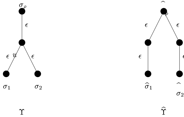
Figure 7: \Upsilon is dominated by \hat{\Upsilon} .
