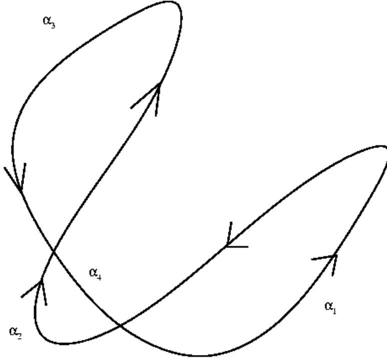
FIGURE 1. Extracting a simple loop with negative action: \alpha_1 , \alpha_3 and \alpha_2 * \alpha_4 are simple loops. One of them should have negative action.
