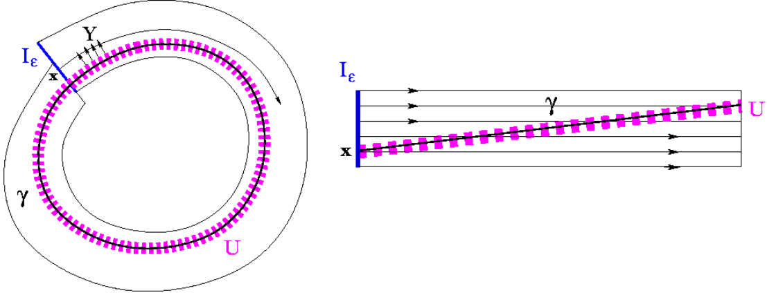
FIGURE 2. Proof of Proposition 2.1
