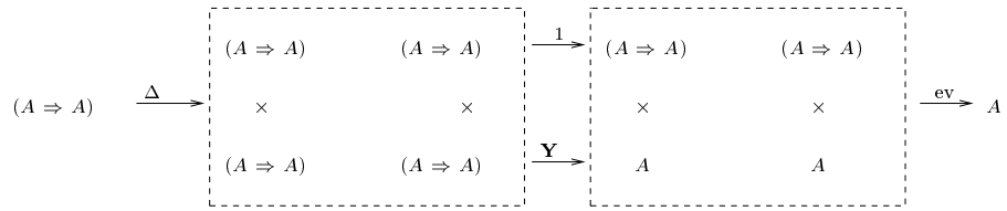
FIG. 8. Composition of maps \Delta; \mathbf{1} \times \mathbf{Y}; \text{ev} .
