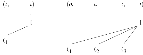
FIG. 6. Trees of questions of arenas (l, l) and (o, l, l, l) .
