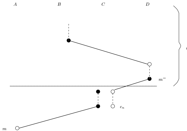
FIG. 5. Composition of strategies is associative.
