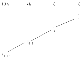
FIG. 15. Tree of questions of arena ((l, l), l, l) .
