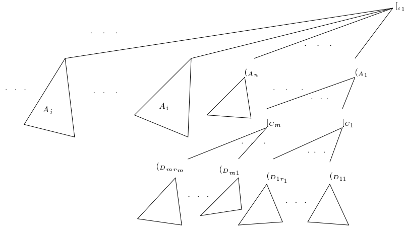
FIG. 17. Forest of questions of arena A .
