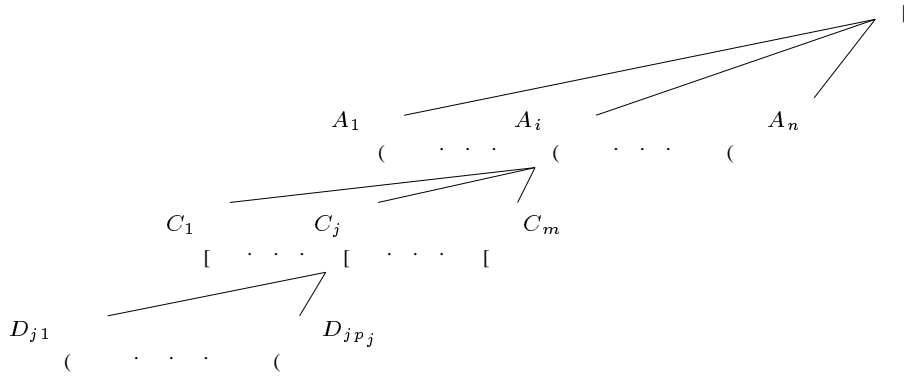
FIG. 10. Shape of arena A .
